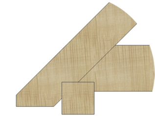
Cold deck detail
