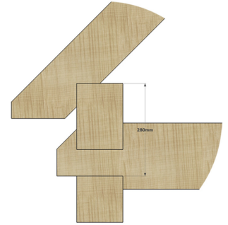
Raised Plate Detail
